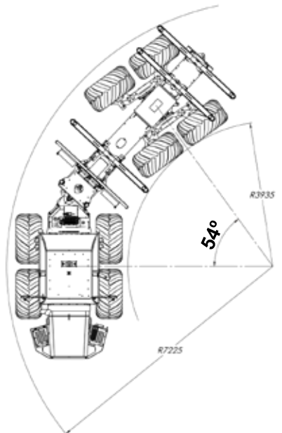
ARTICULATED WAGON
