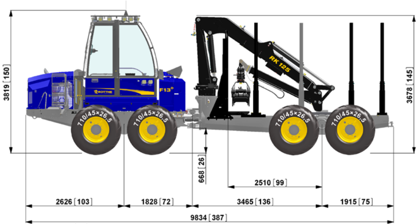
STANDARD WAGON
